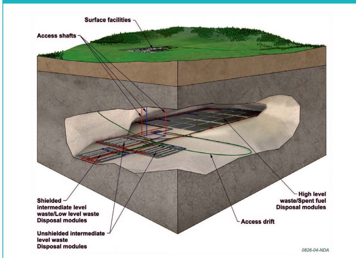
Figure 3.3: Possible design for a GDF in higher strength rock
