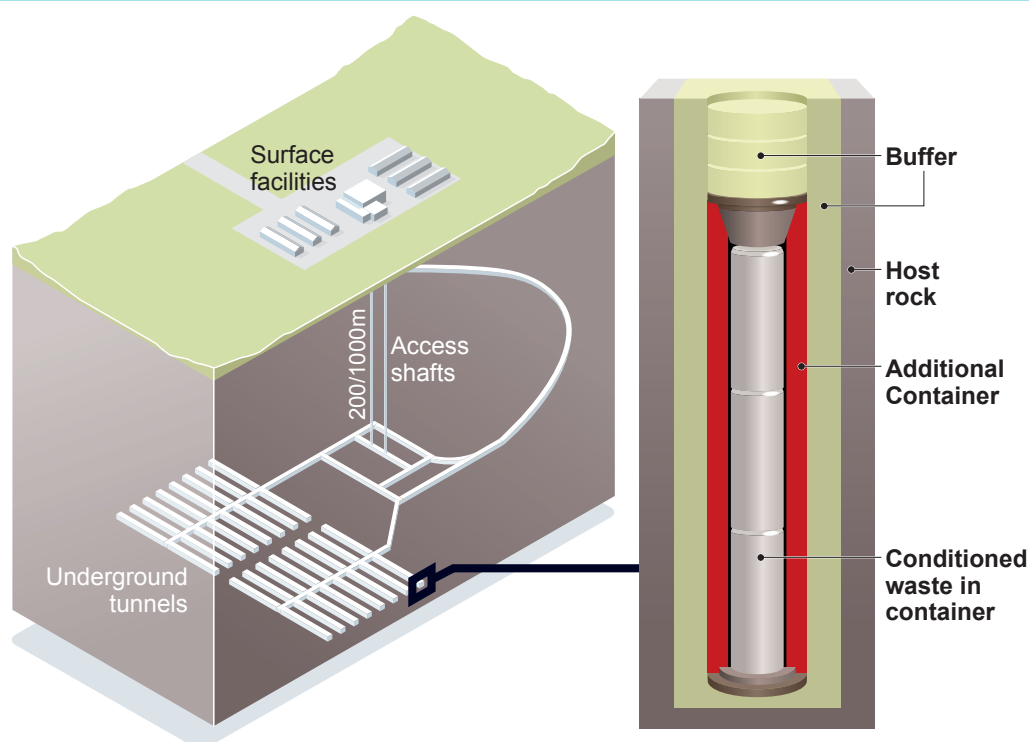
Figure 8.1: Multi-barrier illustration/cross section
