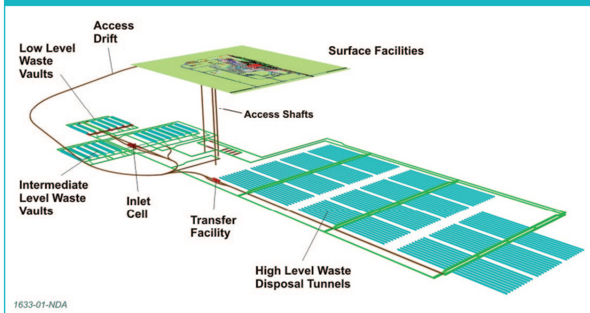
Figure 9.1: Generic design for a GDF (image provided by the NDA)
